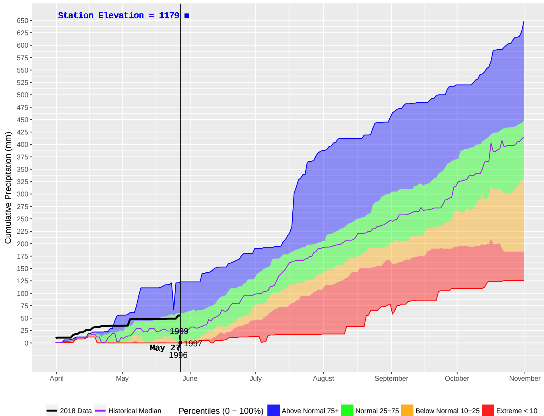
HOLMES (201) : Historical (1987–2016) and Current (2018) Noon Cumulative Precipitation
