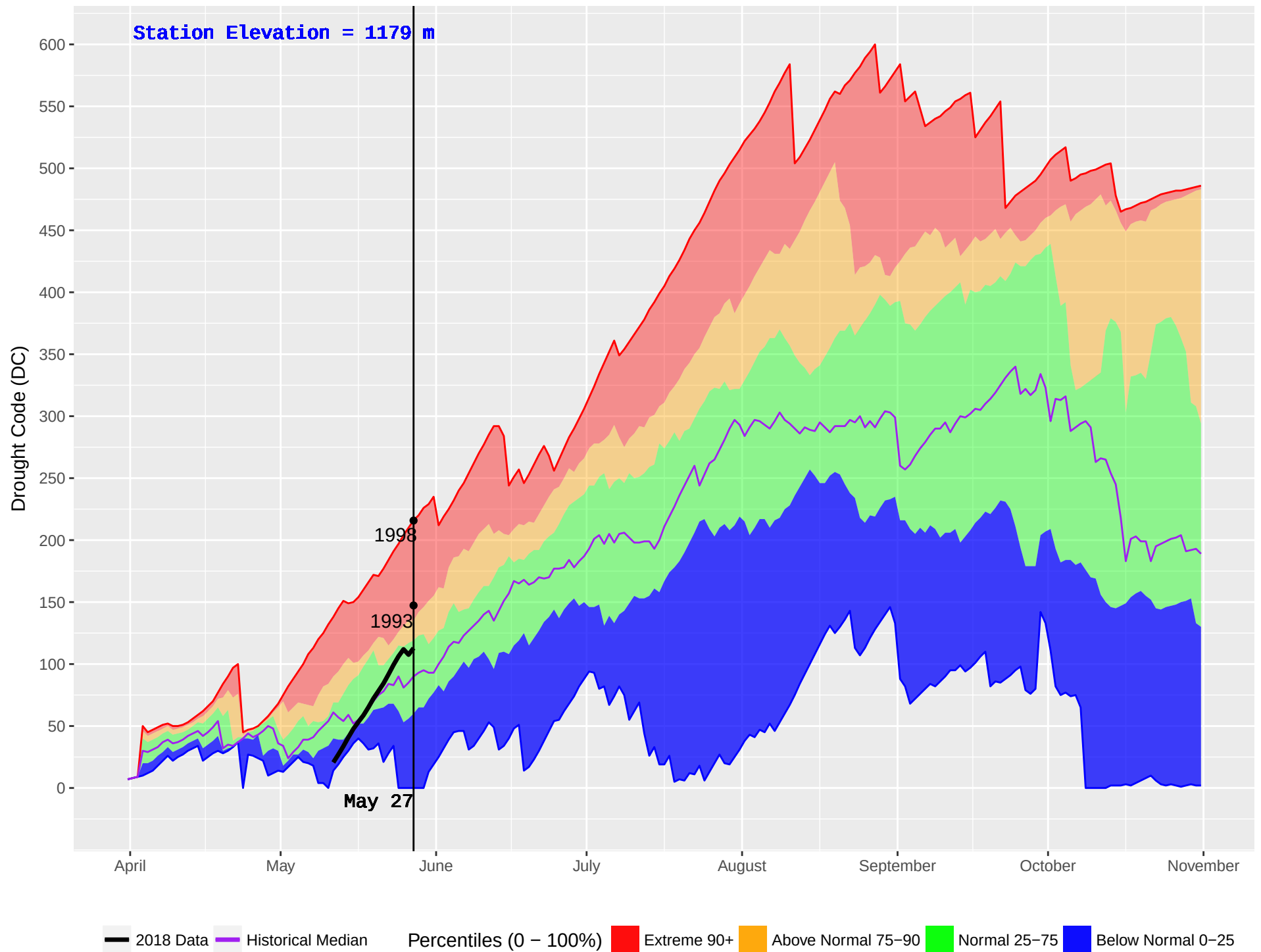
HOLMES (201) : Historical (1987–2016) and Current (2018) Noon Drought Code (DC)
