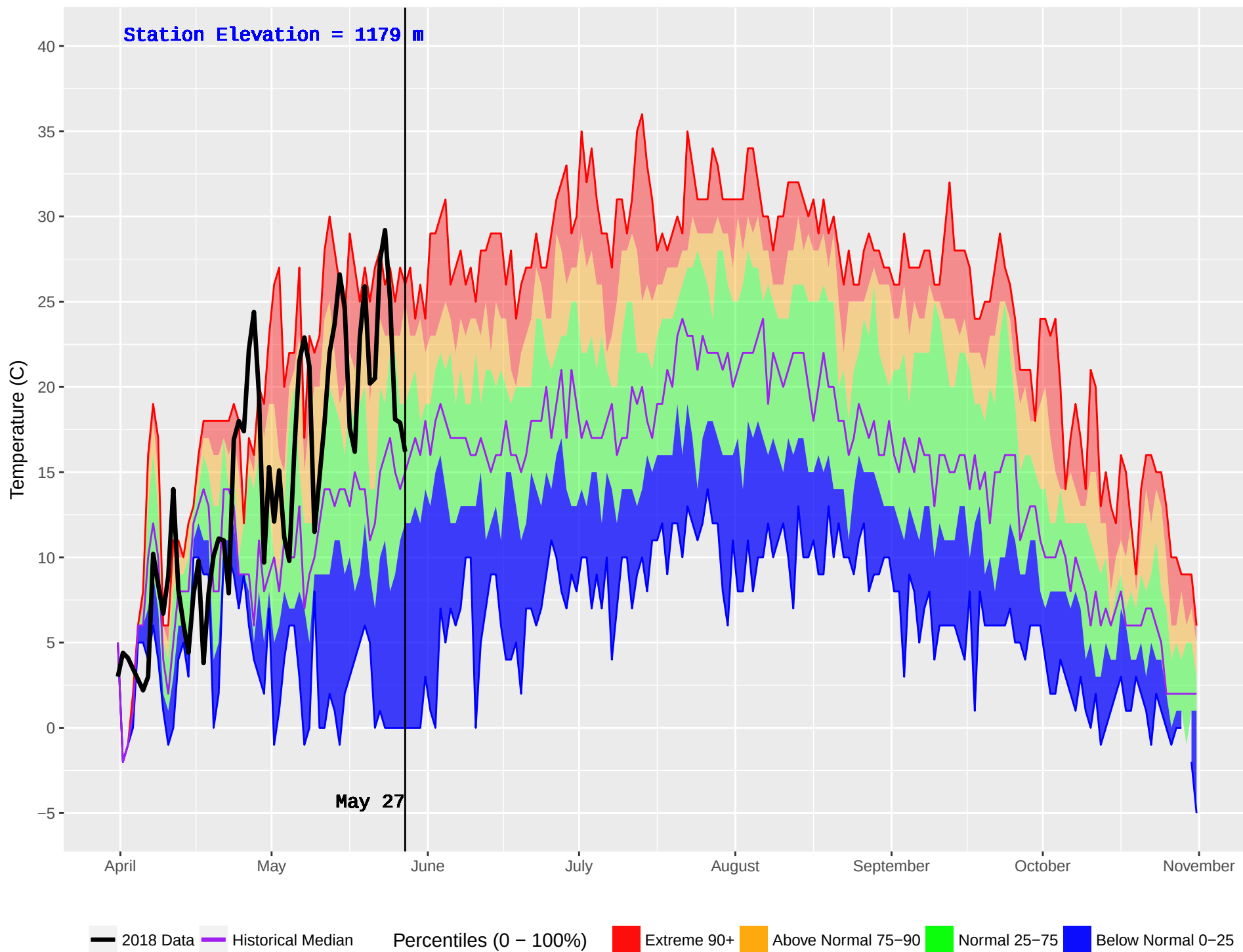
HOLMES (201) : Historical (1987–2016) and Current (2018) Noon Temperature
